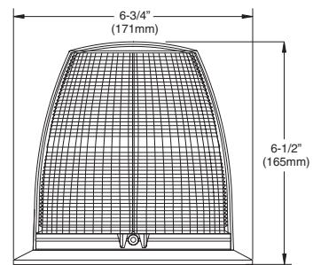
Aerodynamic Dome
