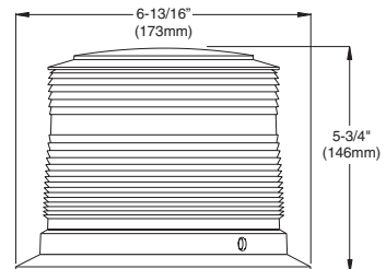
Low Dome
